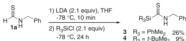
Scheme 3. Reaction of thioformamide 1a with LDA and \text{PhMe}_2\text{SiCl} and t\text{-BuMe}_2\text{SiCl} .
