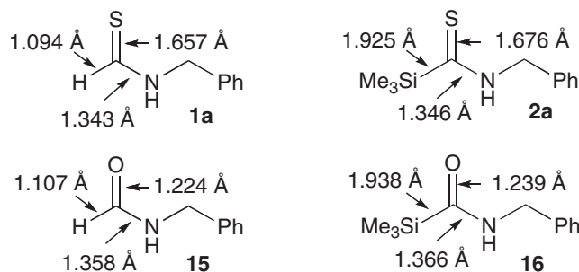
Figure 1. Bond distances of optimal structures of compounds 1a , 2a , 15 , and 16 at the B3LYP/6-31+G(d) level.
