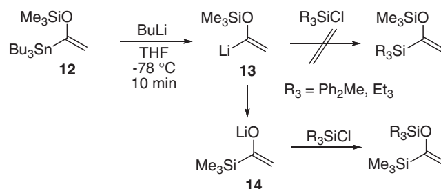
Scheme 7. Reverse Brook rearrangement of siloxyvinyl-lithium 13 .
