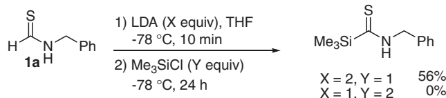
Scheme 6. Reaction of 1a with different amounts of LDA and Me 3 SiCl.
