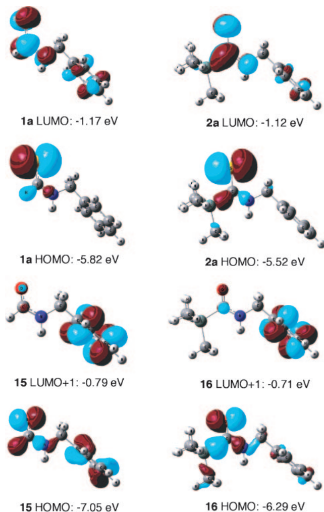
Figure 2. Energy levels of HOMO and LUMO or LUMO+1 of compounds 1a , 2a , 15 , and 16 at the B3LYP/6-31+G(d) level.
