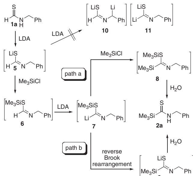
Scheme 4. Plausible reaction pathway.
