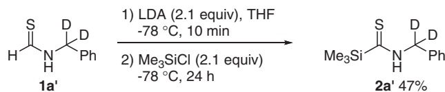
Scheme 5. Reaction of deuterated thioamide 1a' .
